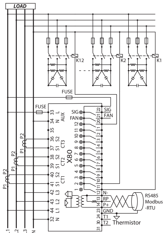
X80 Connection diagram for 3 Phase 12 Step model
