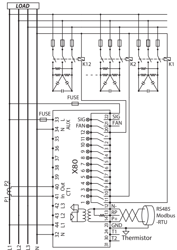
X80 Connection diagram for 1 Phase 12 Step model
