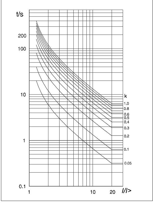
Long-time Inverse
