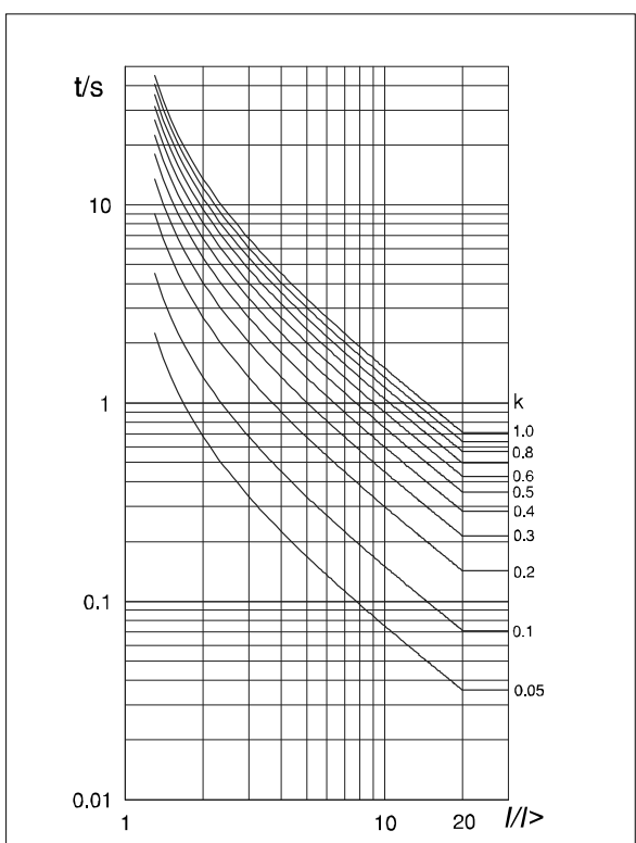
Very Inverse
