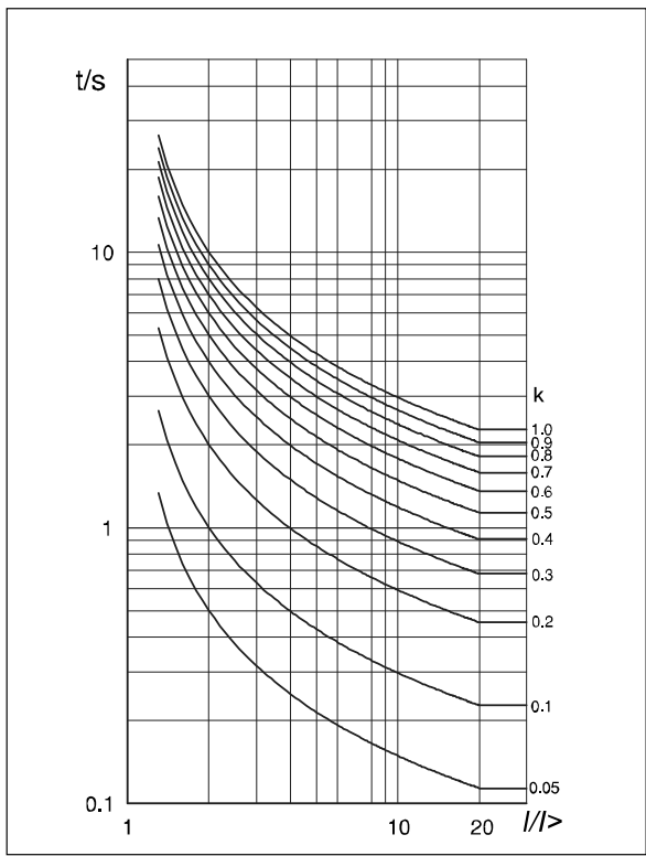
Normal Inverse
