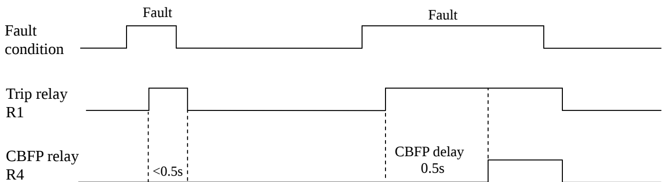
Timing diagram for CBFP. (R4 function set to CBFP, delay 0.5s.)
