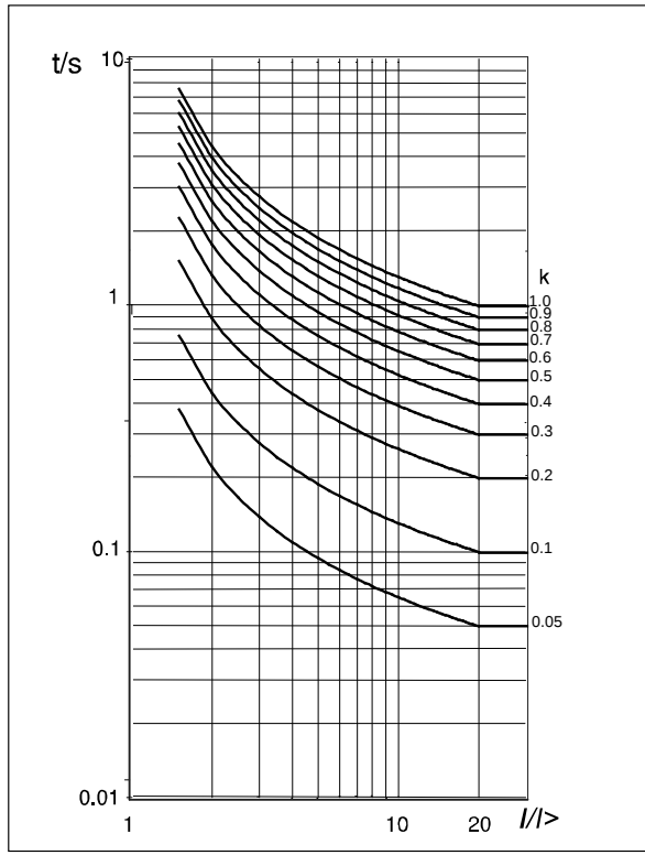
Normal Inverse 1.3/10
