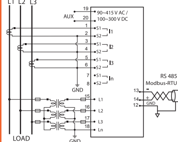
3-PHASE 3-WIRE SYSTEM: 3CTs, 3VTs
