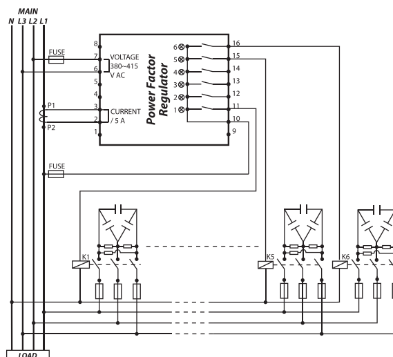
Diagram 2 - For model PFR96P
