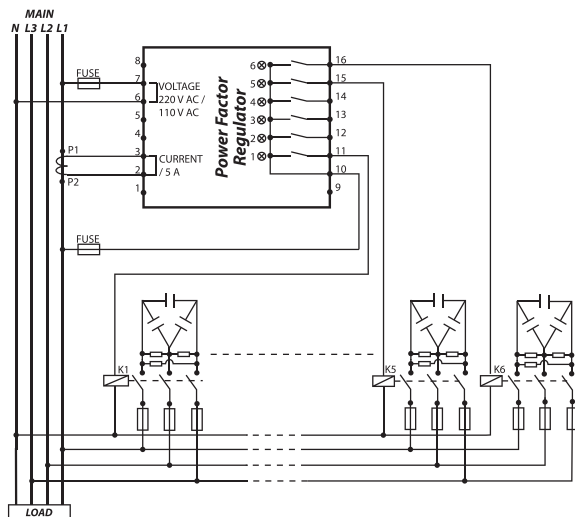
Diagram 1 - For model PFR96
