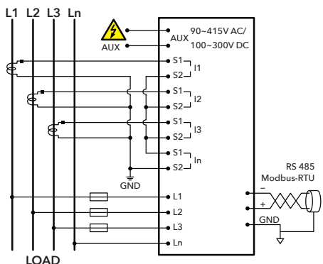
3-PHASE 4-WIRE SYSTEM: 3CTs, direct V input
