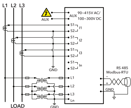
3-PHASE 3-WIRE SYSTEM: 3CTs, 3VTs
