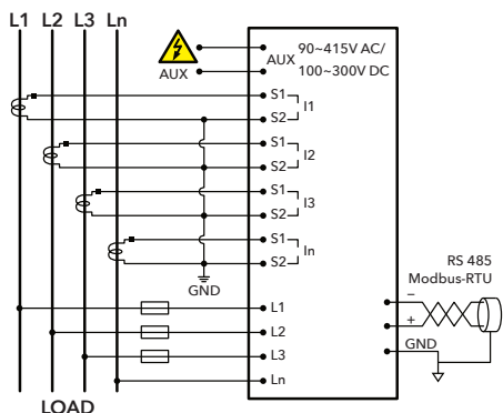
3-PHASE 4-WIRE SYSTEM: 4CTs, direct V input
