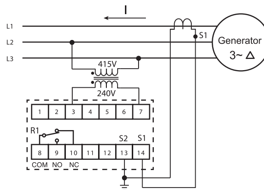
3-Phase 3-wire system
