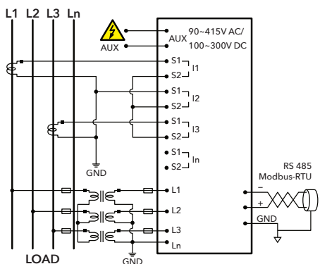
3-PHASE 3-WIRE SYSTEM: 2CTs, 3VTs
