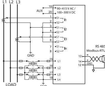
3-PHASE 3-WIRE SYSTEM: 2CTs, 3VTs
